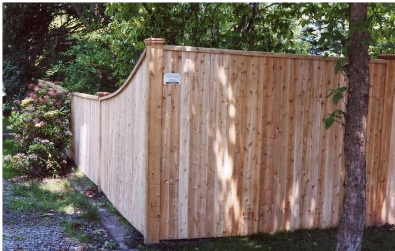
Outside of fence. Fence dowelled into cedar 5x5 posts
